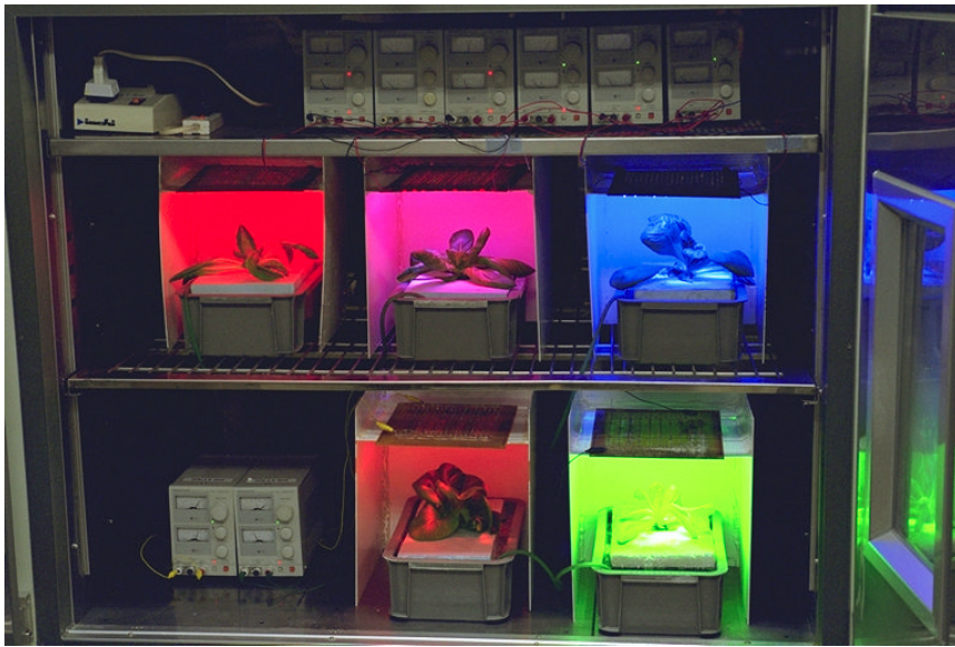
Figure 16.7. Experiments at Tokai University Plant Factory Laboratory growing plants under different colored LED lights. Photo courtesy M. Takatsuji, Dept. of Biology, Science and Technology, Tokai Univ.
