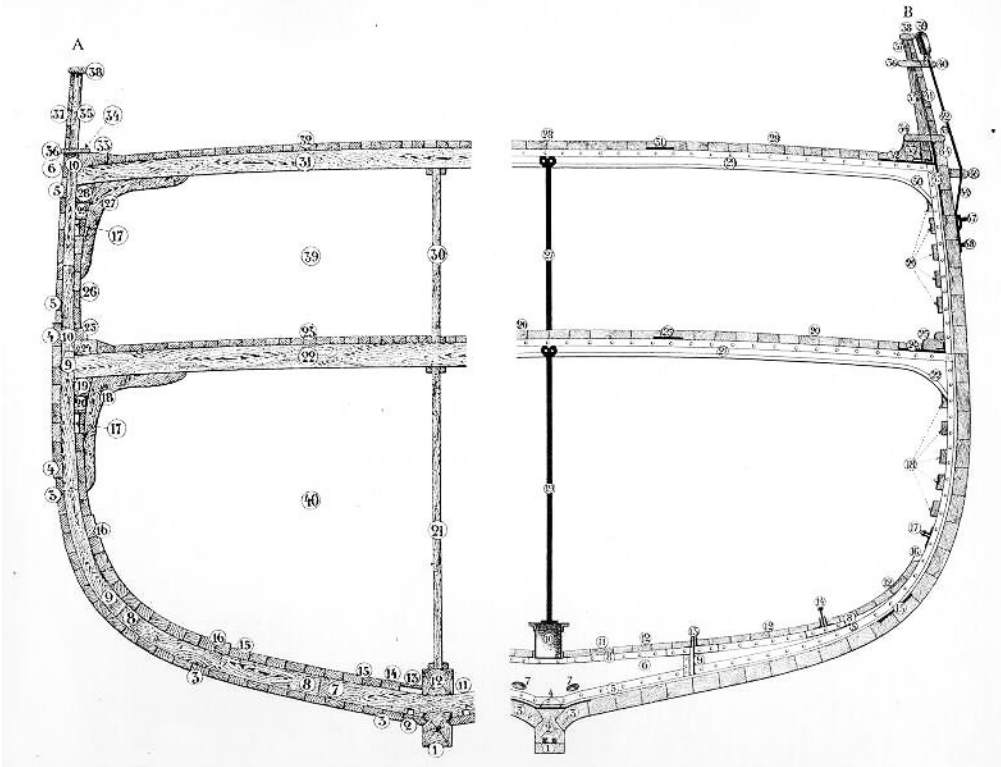
Figure 7.1. Cross section of a wooden hull (left), and a 19 th century hull incorporating some iron parts (right). From Baker, W., The Lore of Ships . 1963: Holt, Rinehart and Winston, “The Hull,” p. 19.
